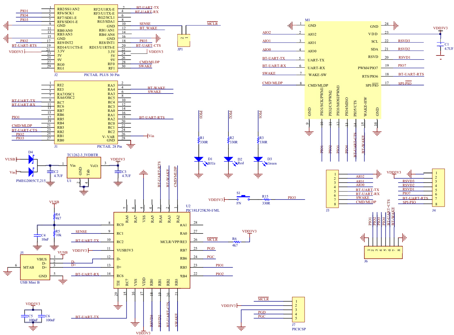
FIGURE 5-1: RN4020 TYPICAL APPLICATION SCHEMATICS
