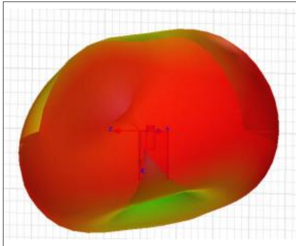
FIGURE 7-3: 3D RADIATION PATTERN AND ANTENNA ORIENTATION
